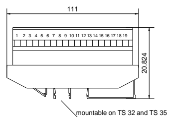
Dimensional drawing PS 47-1-08
