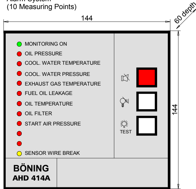
Built-in housing for panel cut-out 138mm x 138mm
