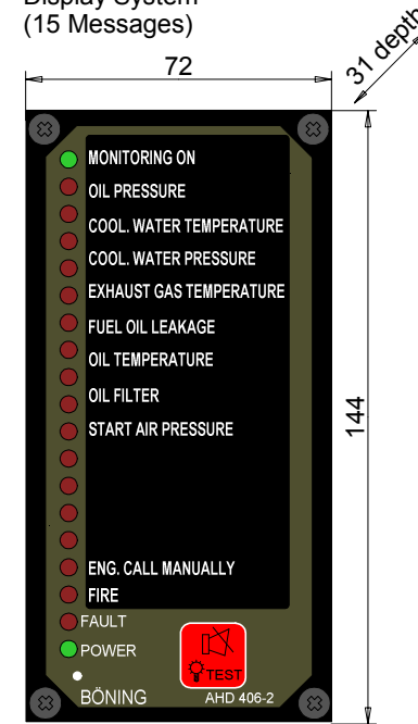
Device for flush mounting (panel cut-out 131 x 61mm)
